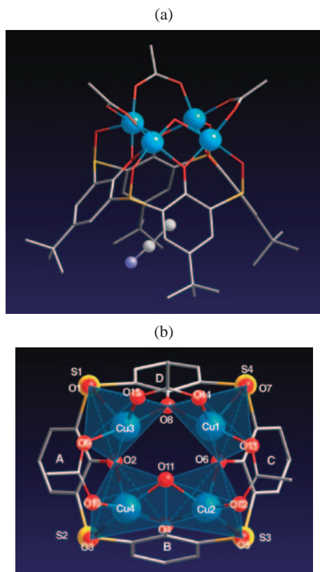
Fig. 2. Crystal structure of [Cu^{II}_4(L^{recc})(OAc)_3(\mu-OH)] ( 2 ). (a) Side view and (b) top view showing the copper(II) coordination polyhedra. tert -Butyl groups are omitted in (b).
