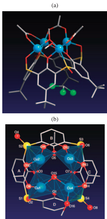
Fig. 1. Crystal structure of [Cu II 4 (L rtet )(OAc) 3 (μ-MeO)(MeOH)] ( 1 ). (a) Side view and (b) top view showing the copper(II) coordination polyhedra. tert -Butyl groups are omitted in (b).
