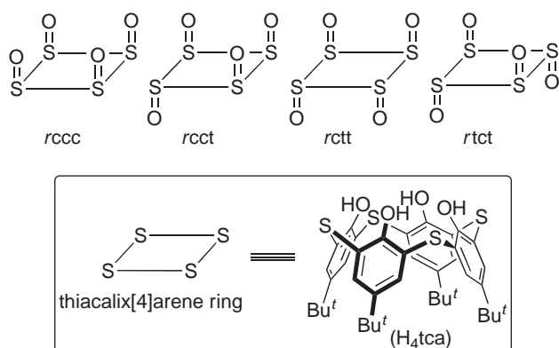
Scheme 2. p -tert-Butylthiacalix[4]arene ring and four stereoisomers of p -tert-butylsulfinylcalix[4]arene, \text{H}_4\text{L} . Herein, we use the term cis (c) or trans (t) to denote the disposition of sulfoxide oxygen with respect to reference oxygen from the mean plane containing four sulfur atoms. The isomer notation proceeds around the system from reference oxygen, which should be chosen to maximize the number of cis arrangements, and cis is preferable to trans .
