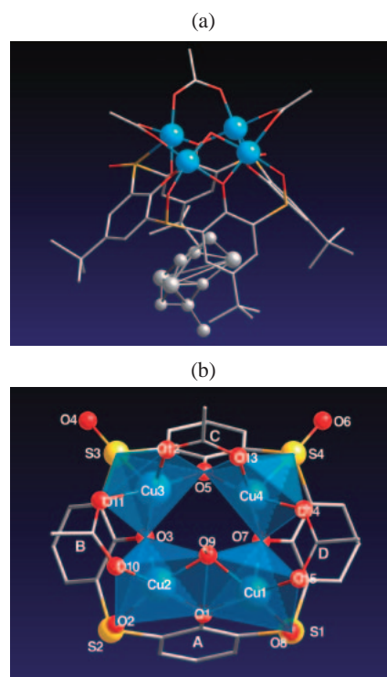
Fig. 3. Crystal structure of [Cu^{II}_4(L^{rett})(OAc)_3(\mu-OH)] ( 3 ). (a) Side view and (b) top view showing the copper(II) coordination polyhedra. tert -Butyl groups are omitted in (b).
