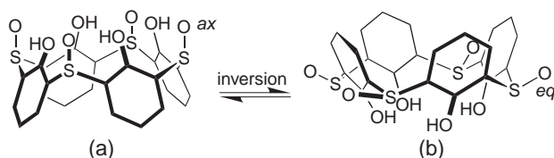
Scheme 4. Ring inversion of H_4L^{recc} between cone-shaped isomers having (a) axial and (b) equatorial sulfinyl oxygen. Double bonds and tert -butyl groups are omitted for clarity.
